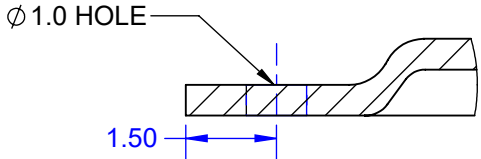
DETAIL E SCALE 8 : 1
